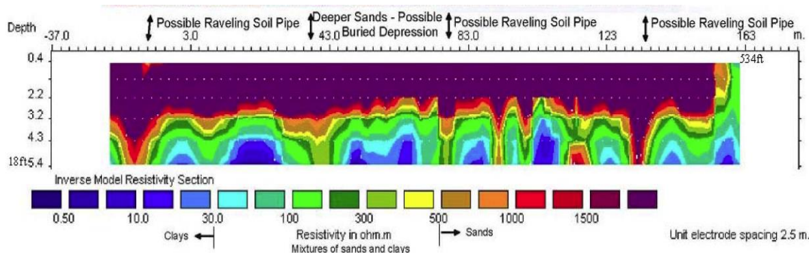
Figure 2-3. Example CCR survey results (Garman and Purcell 2004).
