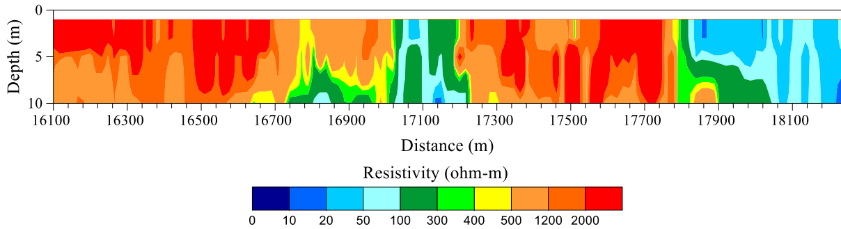
Figure 3-6. Sample resistivity profile generated by Surfer.
